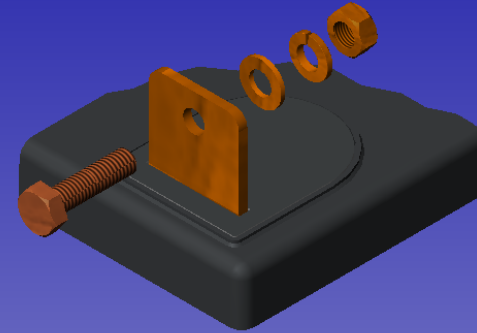
L-Blade Terminal (Solid Copper) M8 Hardware
